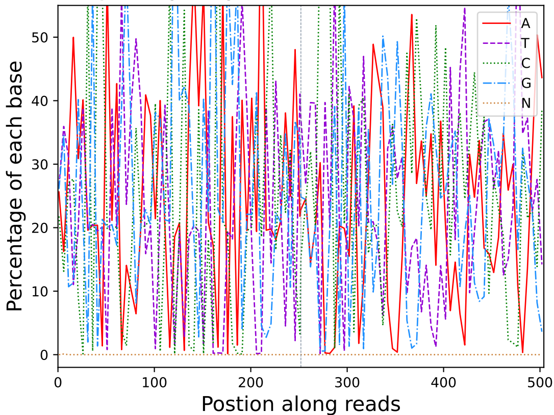
Base percentage along reads (R10106)
